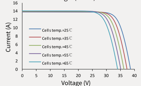
Current-Voltage (430W)
